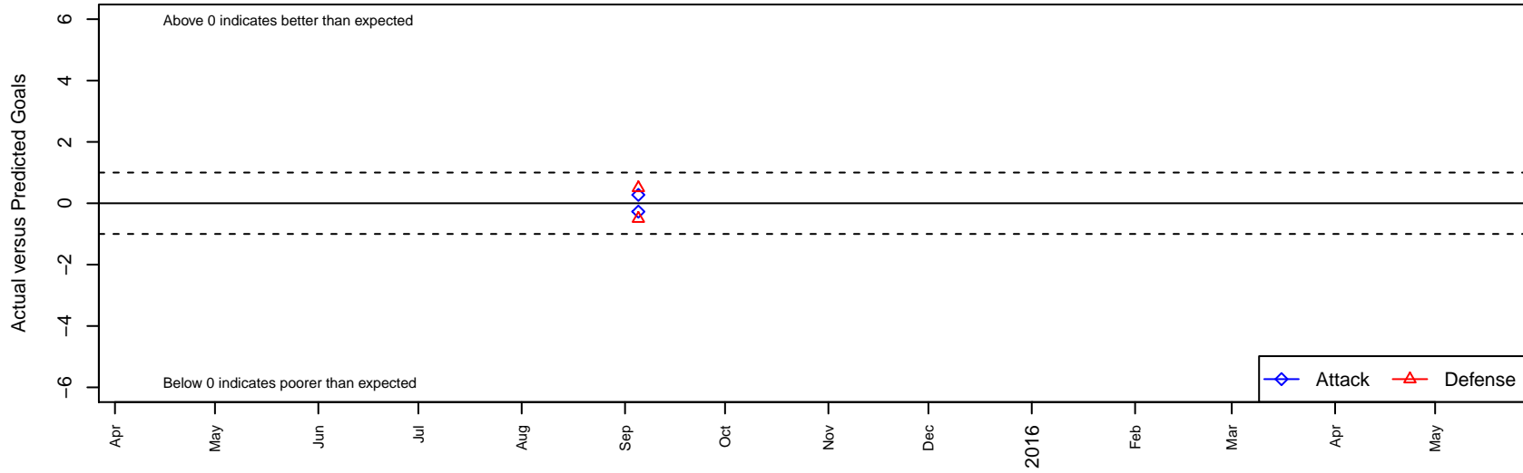
Coquitlam Metro Ford Extreme 2000G Dots are actual minus expected GF (blue circles) and GA (red triangles). Blue line is smoothed change in attack strength. Red is smoothed change in defense strength.
